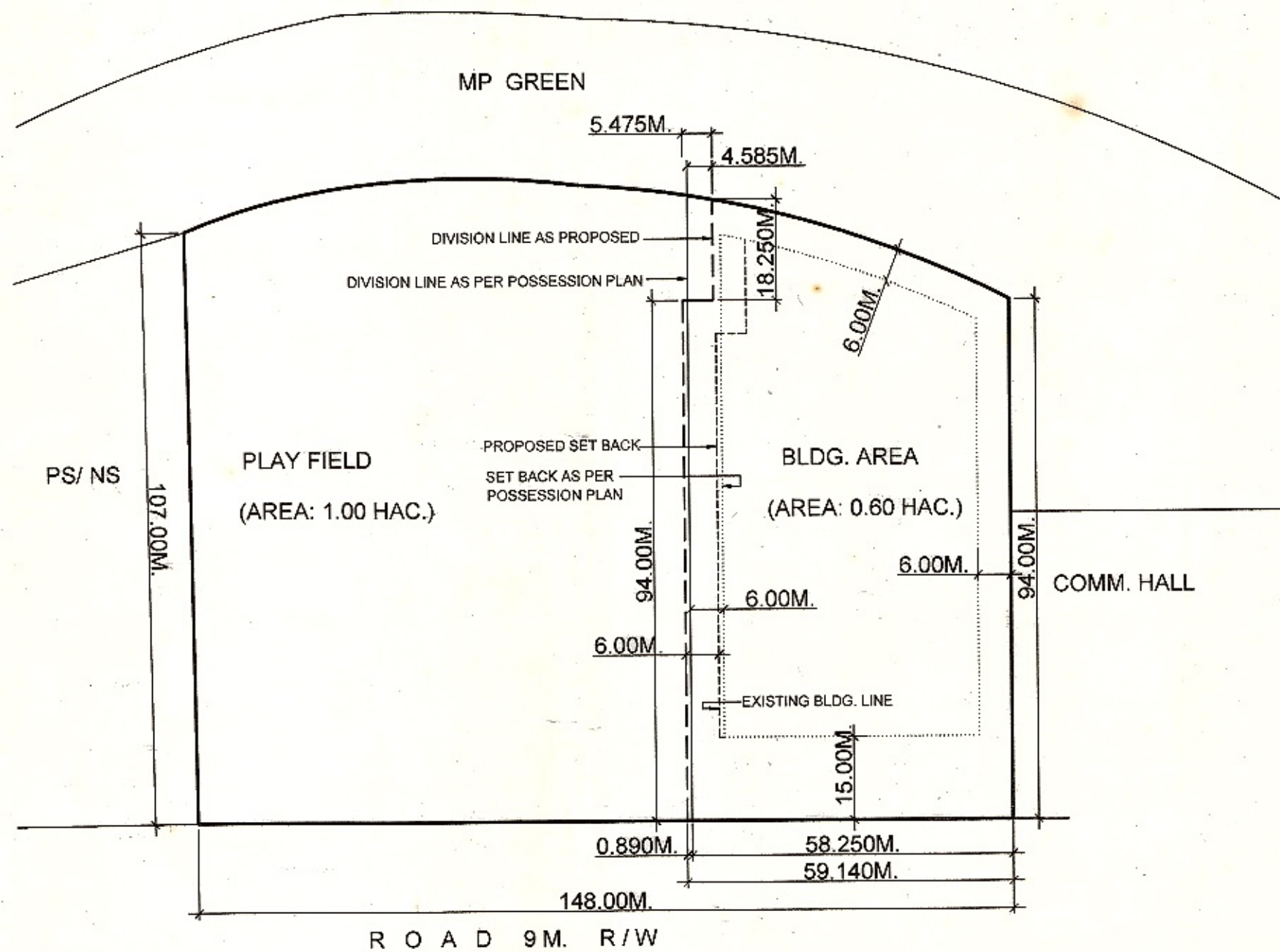
SITE PLAN
